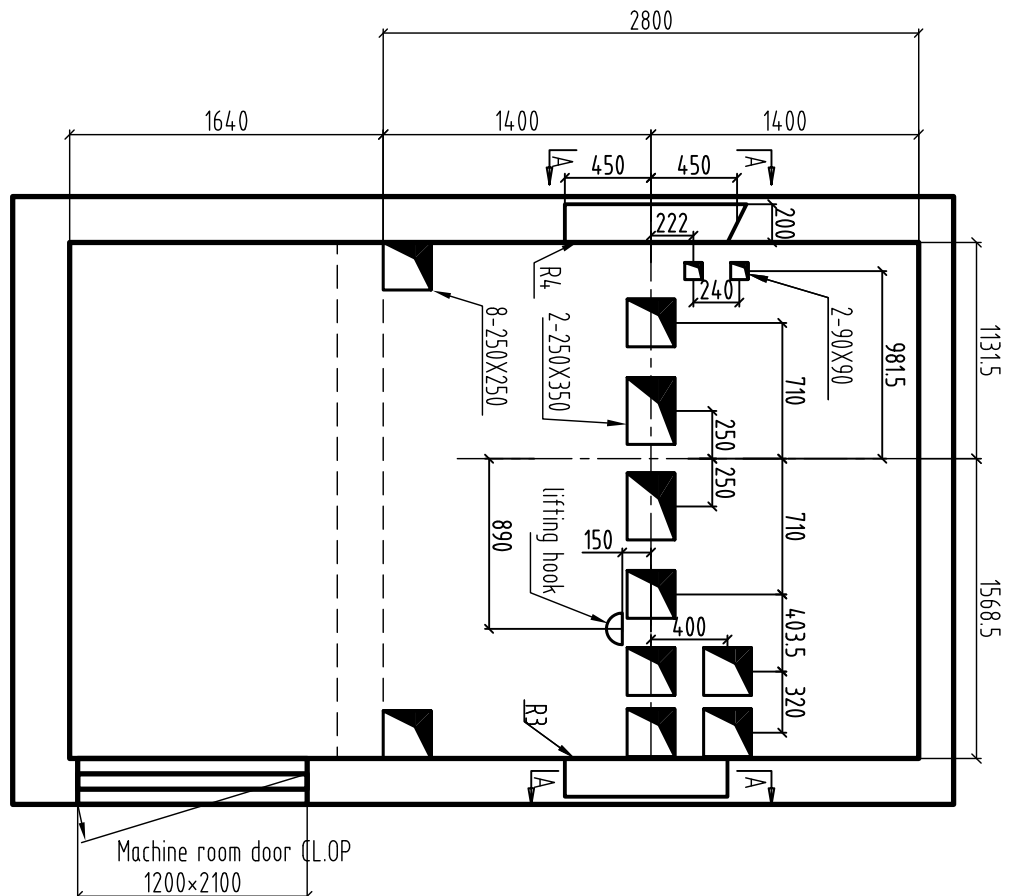
Foreseen hole diagram of machine room
